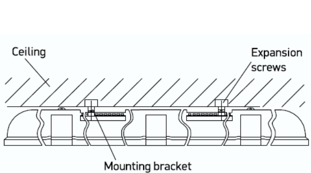
b) Ceiling mounting
